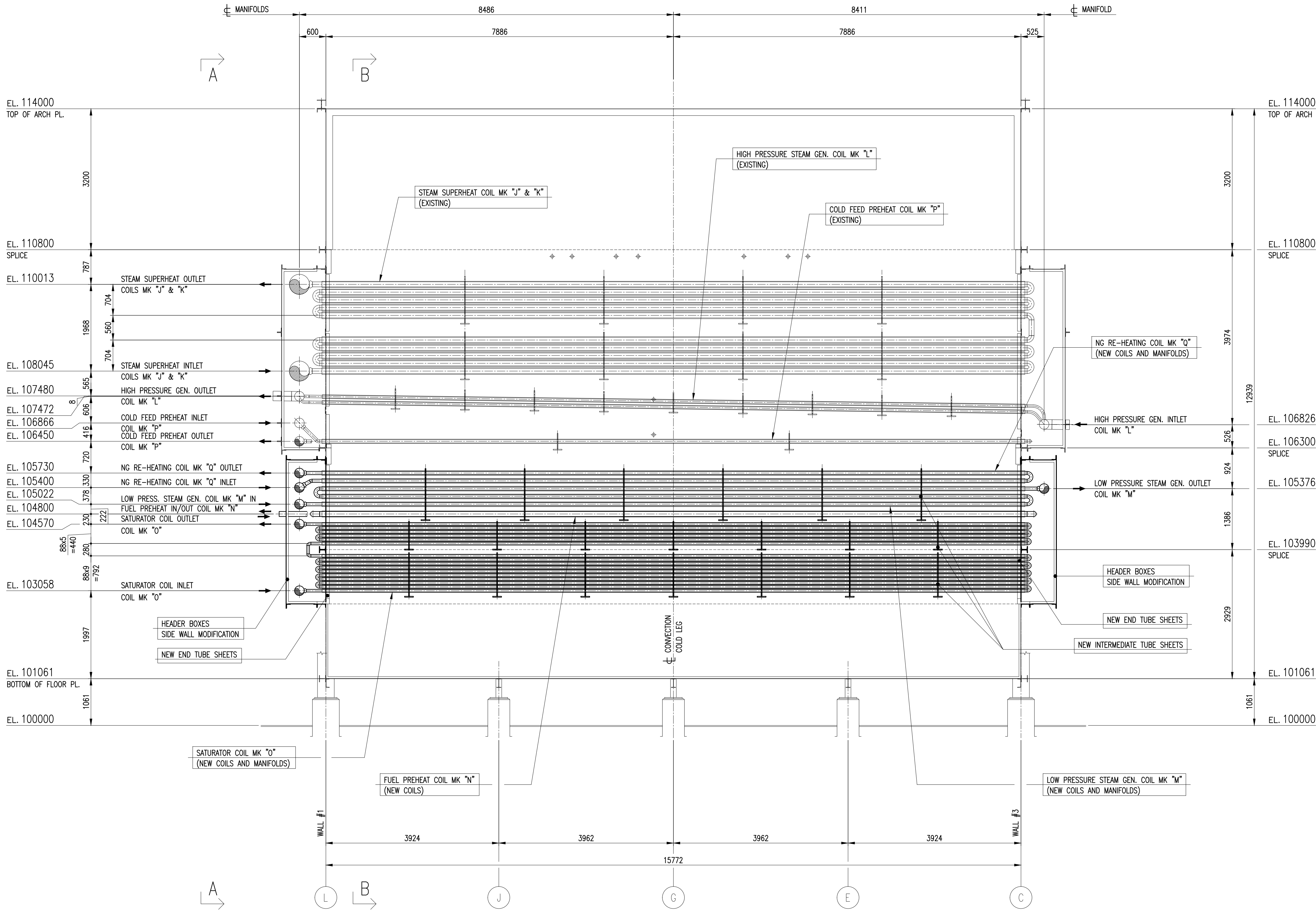
COLD LEG ELEVATION SECTION (LOOKING FROM WALL #8)
