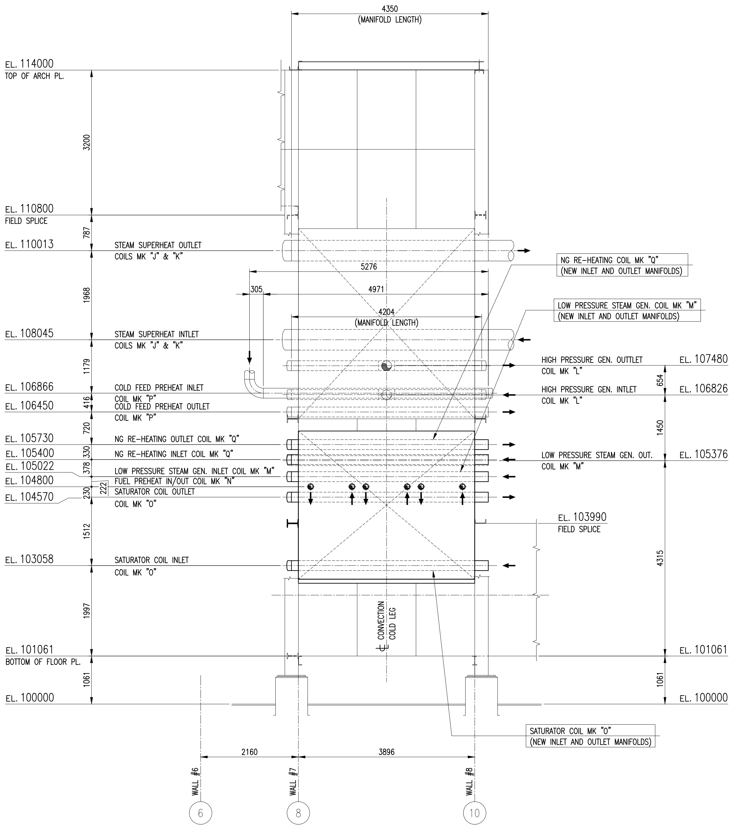
ELEVATION VIEW A-A (LOOKING FROM WALL #1) (SEE DRAWING N° A12140-E-MDH-0003)
