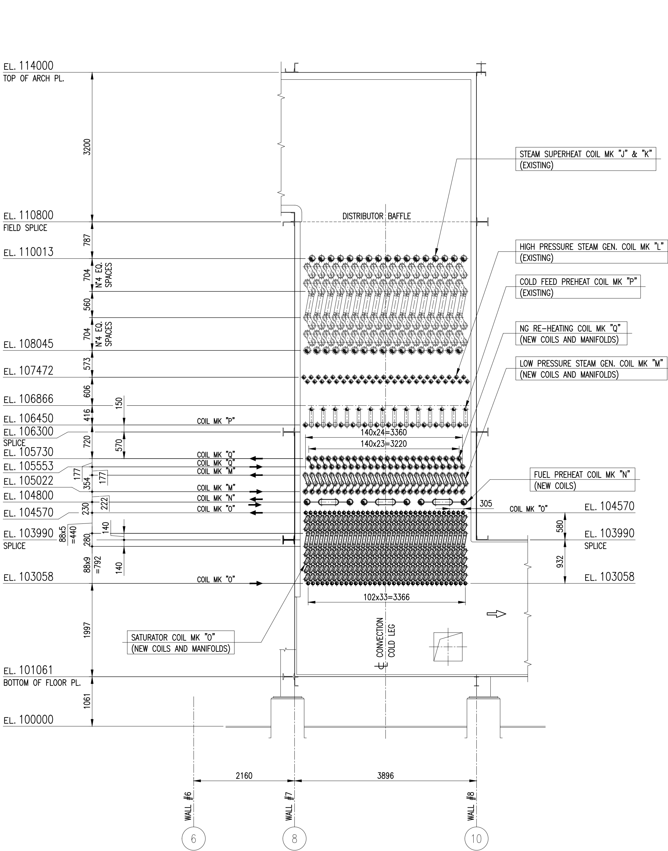
ELEVATION SECTION B-B (LOOKING FROM WALL #1) (SEE DRAWING N° A12140-E-MDH-0003)
